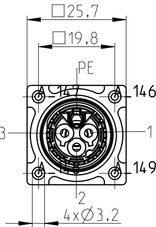
plug face male
