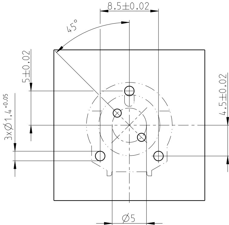
PCB-Layout (advice)
