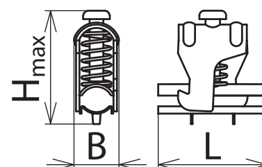
Maßbild SAK 18 AS V4A
