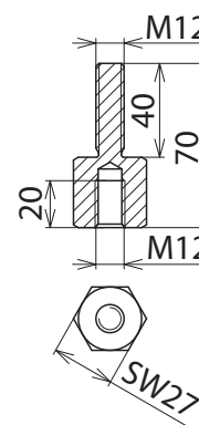
Maßbild AS SCHR M12 M12 40
