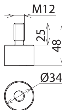
Maßbild AS SCHW M12 25
