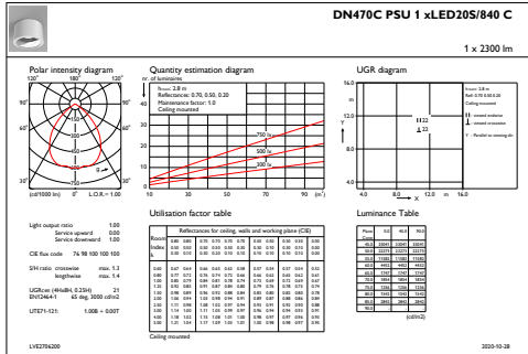
IFGU1_DN470CPSU1xLED20S840C
