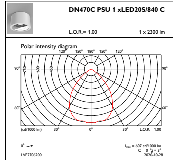
OFPC1_DN470CPSU1xLED20S840C
