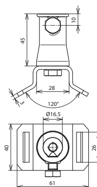
Maßbild AS SPB25 BB16 V2A
