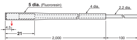
39-E E32-T51F 2M (Free Cutting)
