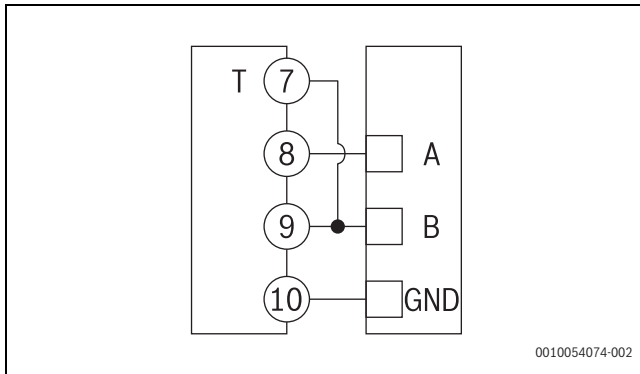
Fig. 104 RS485 Modbus Master diagram
