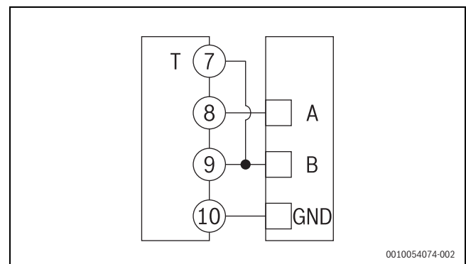
Fig. 123 Diagrama Modbus RS485 maestro
