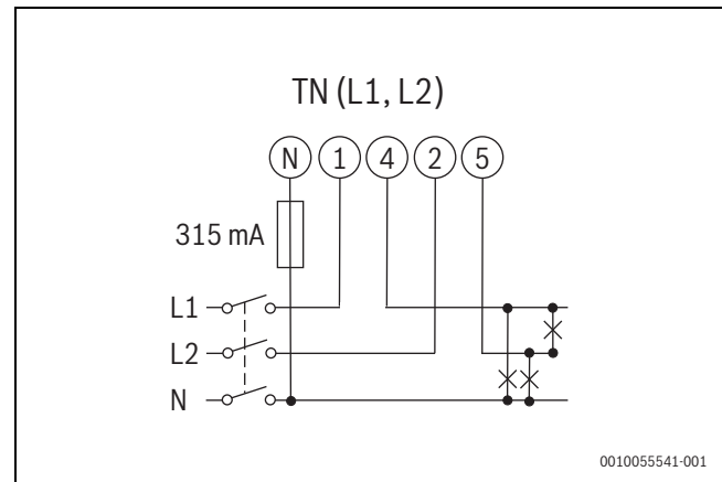
Fig. 101 Two-phase system diagram, 3-wire (TN)
