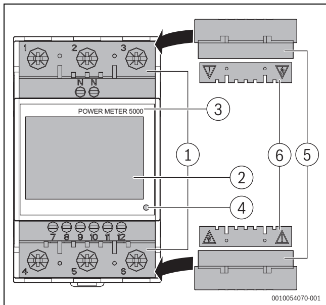
Fig. 97 Product overview
