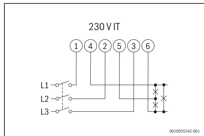
Fig. 102 Three-phase system diagram, 3-wire (230 V IT)
