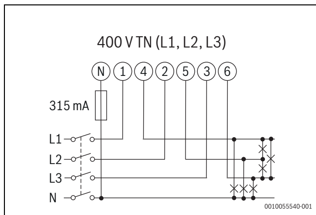
Fig. 100 Three-phase system diagram, 4-wire (400 V TN)
