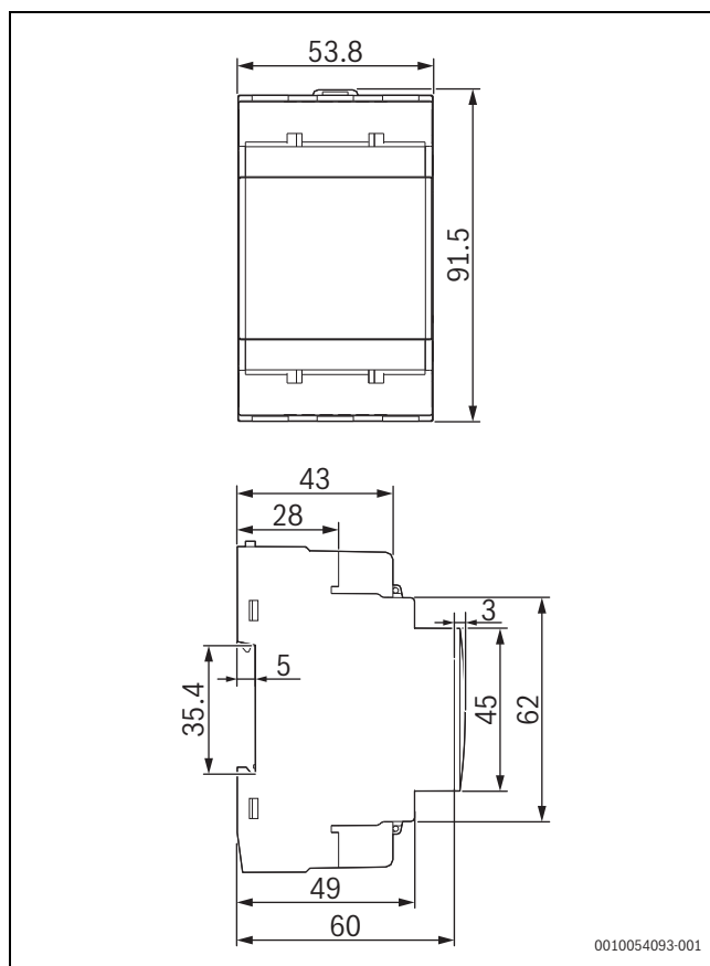
Fig. 99 Product dimensions
