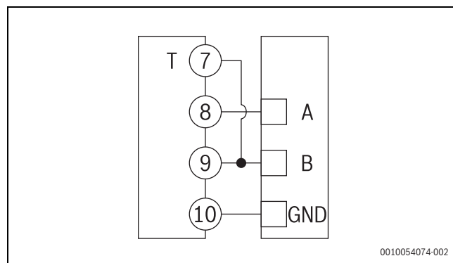
Afb. 294 RS485 Modbus Master schema
