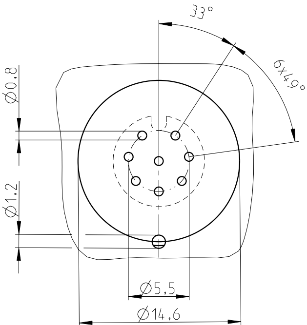
PCB-Layout (advice)
