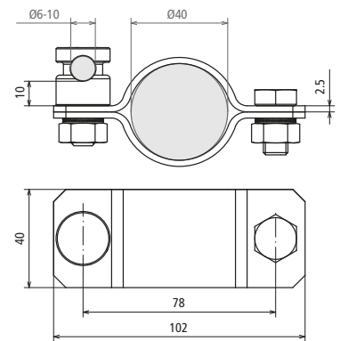
Maßbild AS D40 KSV 6.10 V2A
