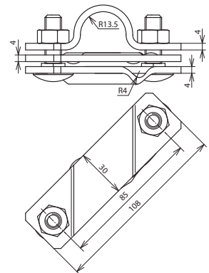
Maßbild AS S RE 27 7.10 FL40 STTZN
