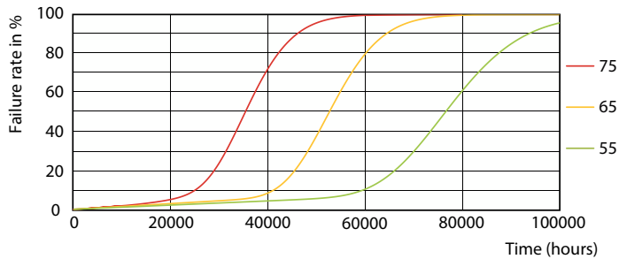
LEDtube-75K-5575-FailureRate-LED
