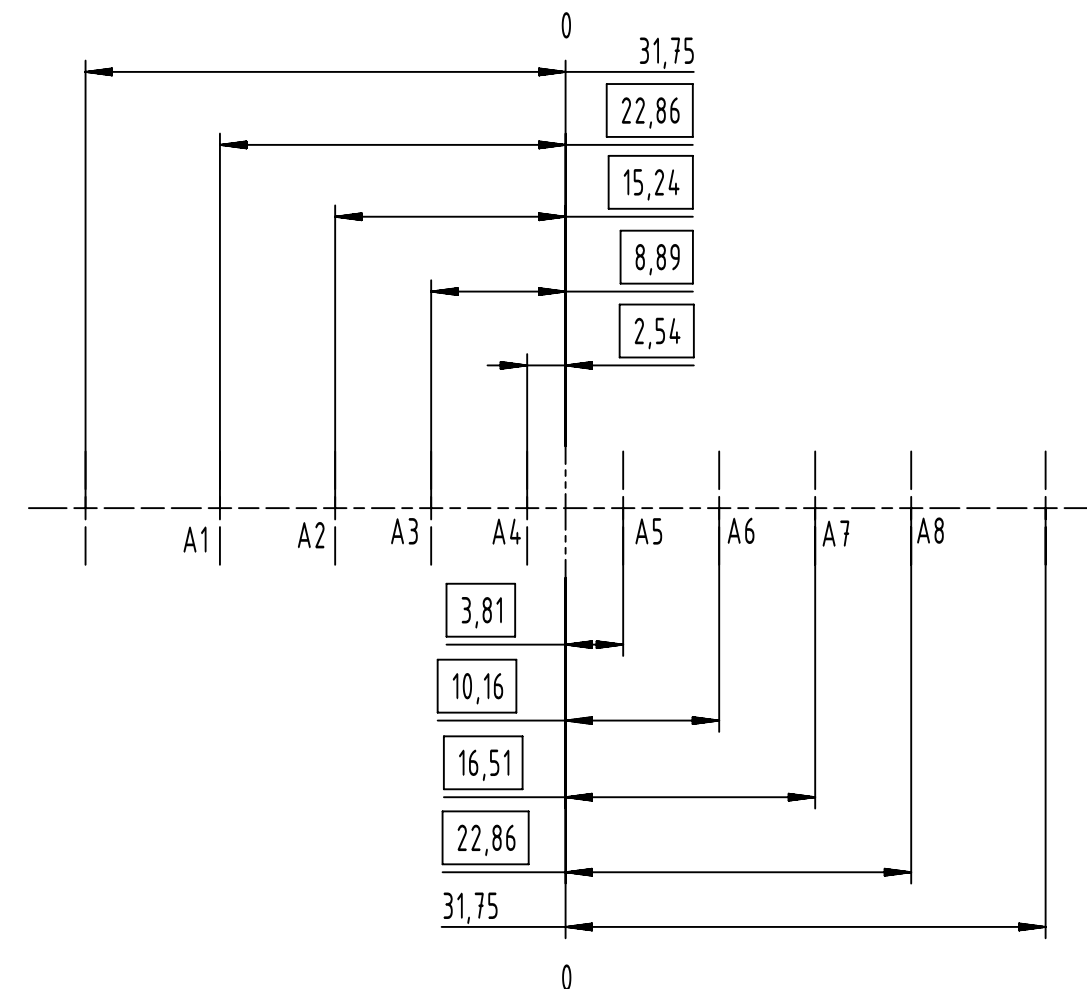
PCB hole pattern, mounting face
