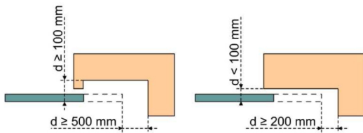
Illustration 2: Safety distance
