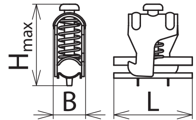
Maßbild SAK 26 AS V4A
