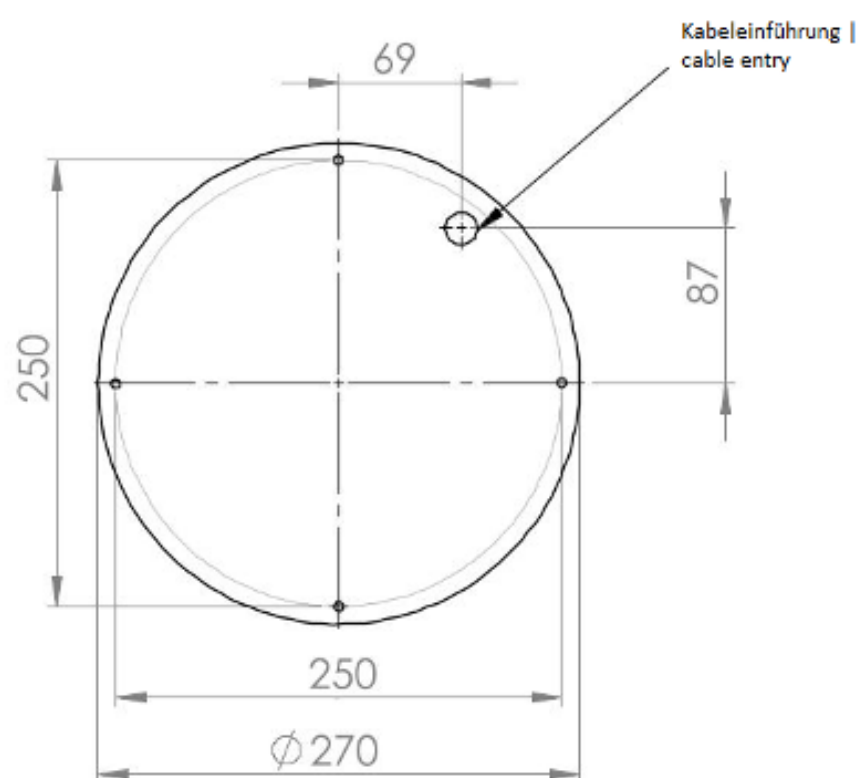
Bohrplan | drilling plan
