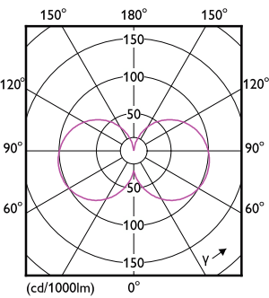
Light Distribution Diagram - CorePro R7S 118mm 7.2-60W 830
