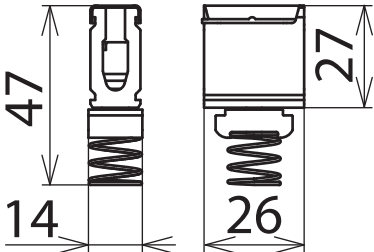
Maßbild AK 16 AS SAK MS
