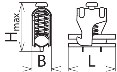
Maßbild SAK 33 AS V4A
