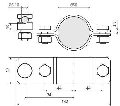
Maßbild AS D50 KSV 6.10 V2A
