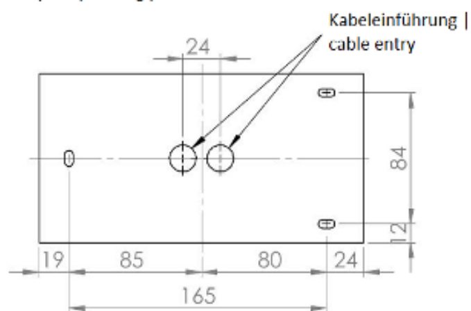
Bohrplan | drilling plan
