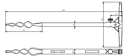
Maßbild EB ASSM5 L350 TGGALZN
