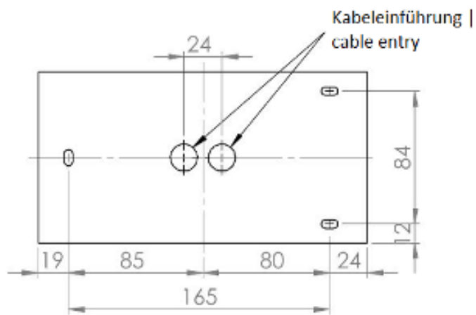
Bohrplan | drilling plan
