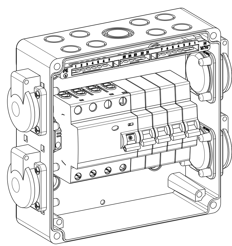
STV 904-K Innenansicht interior view
