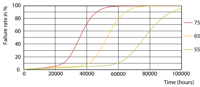
LEDtube-75K-5575-FailureRate-LED
