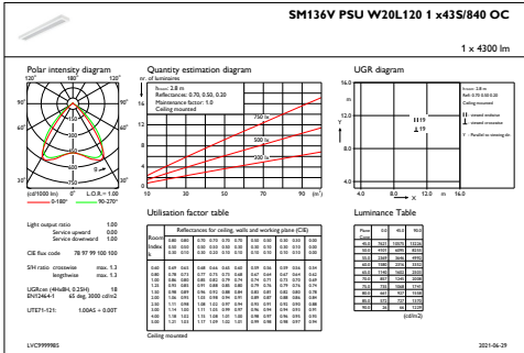
IFGU1_SM136VPSUW20L1201x43S840OC
