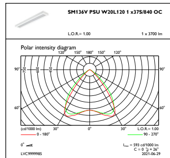
OFPC1_SM136VPSUW20L1201x375840OC
