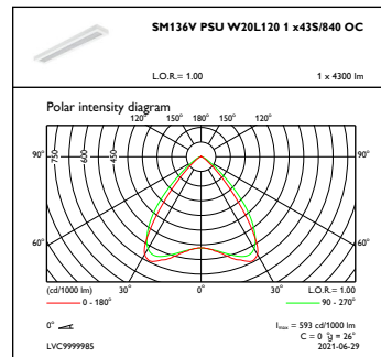
OFPC1_SM136VPSUW20L1201x435840OC
