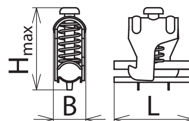
Maßbild SAK 21 AS V4A
