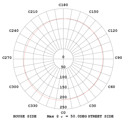
MAX INTENSITY CONE SURFACE DISTRIBUTION DIAGRAM
