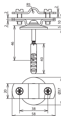
Maßbild LH ZS 7.10 FL30 AS KD8X40 V2A
